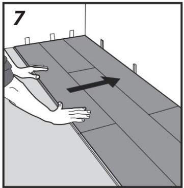
Figure 7 After 3 rows, adjust the expansion gap from the first row to the wall to 10mm+.
