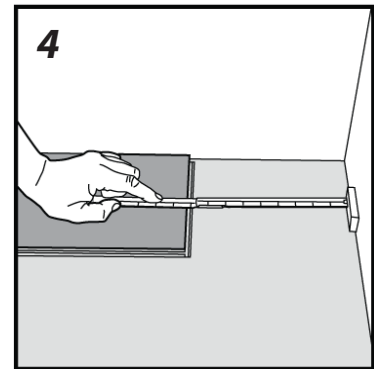
Figure 4 At the end of the first row, measure the length of the last plank, making sure to leave a 10mm expansion gap.
