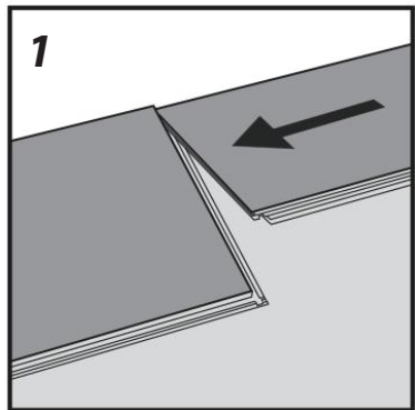
Figure 1 First plank, first row. Start in the left hand corner of the room with the locking strip(groove) facing the room. Remember to leave a 10mm expansion gap between the wall( left) and the board. It is more practical to adjust the expansion gap between the long side and the wall
