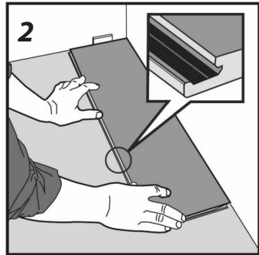
Figure 2 Second plank, first row. Place next floor board tight to the short end of the first plank in the corner.
